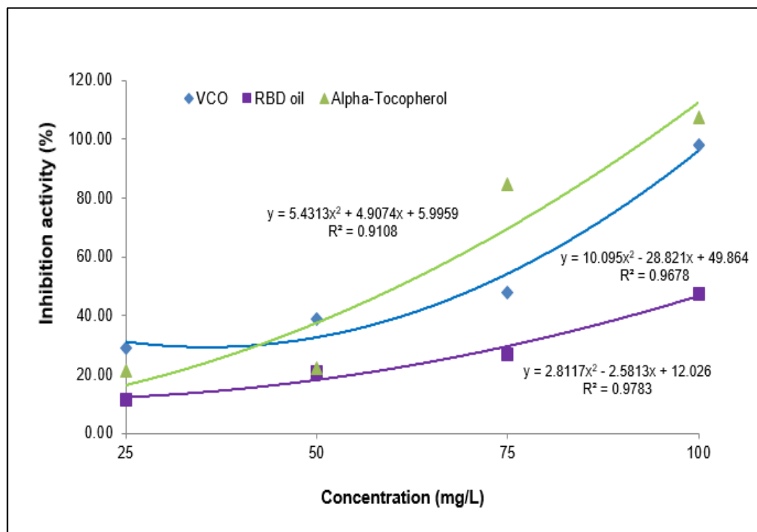
Figure B Antioxidant activity (%) of VCO extract, RBD CO, and standard of \alpha -tocopherol using DPPH assay.
