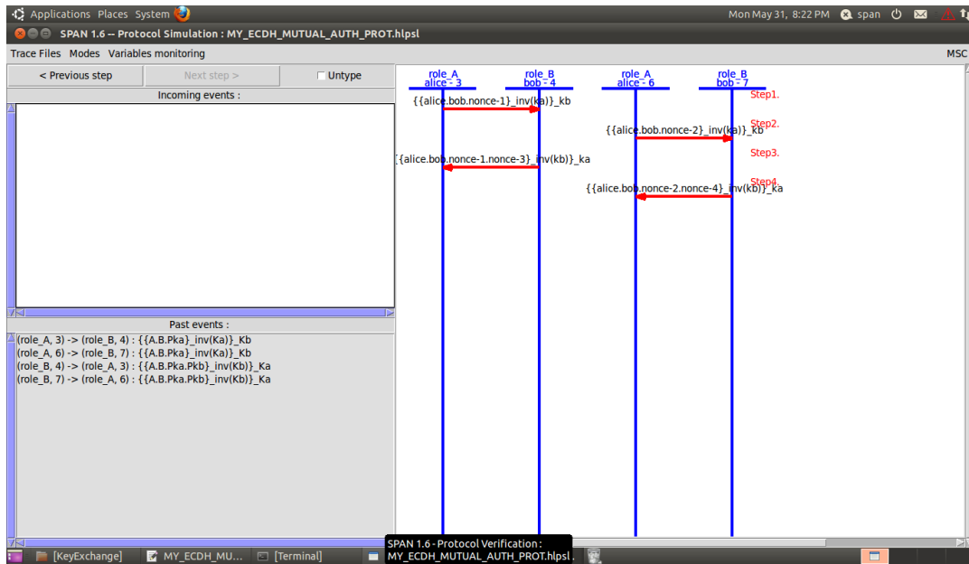
(c)- AVISPA intruder model after successful mutual authentication
