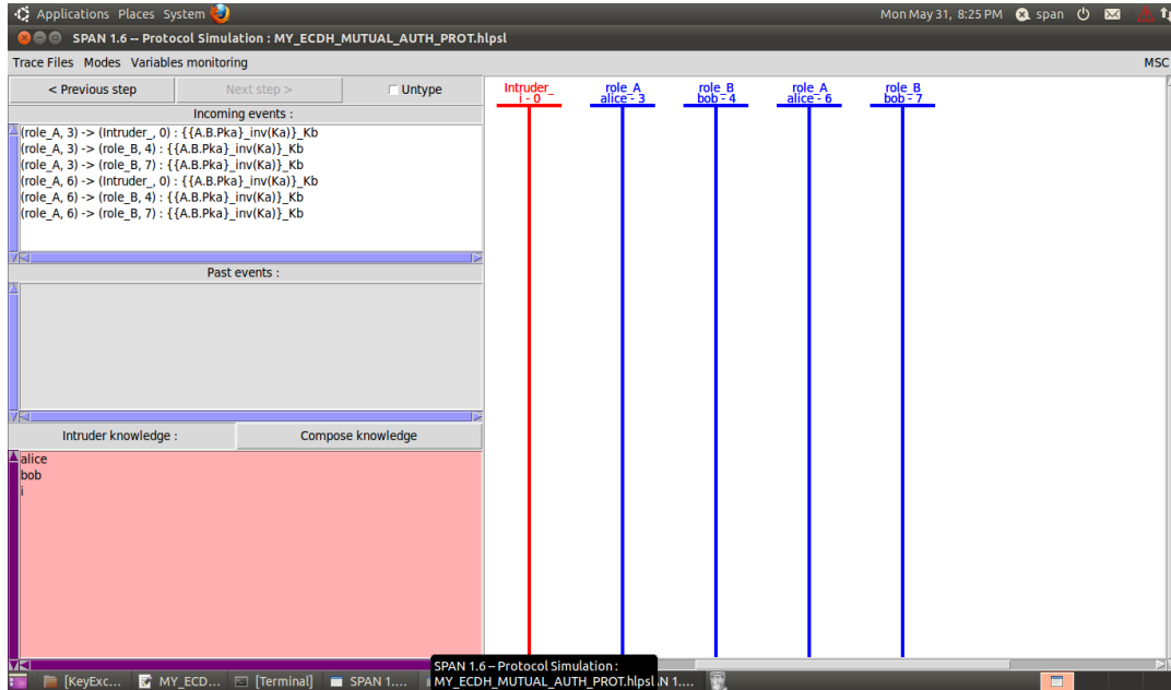
(a) – AVISPA intruder model with OFMC security checker in Step 1
