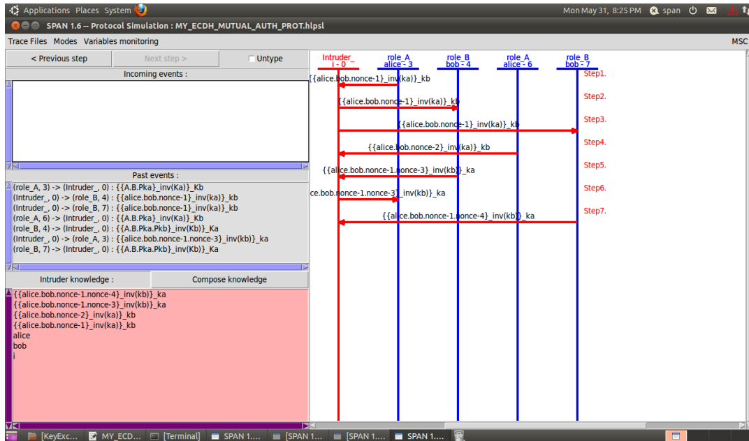
(b) – AVISPA intruder model with ATSE security checker on concluding all steps
