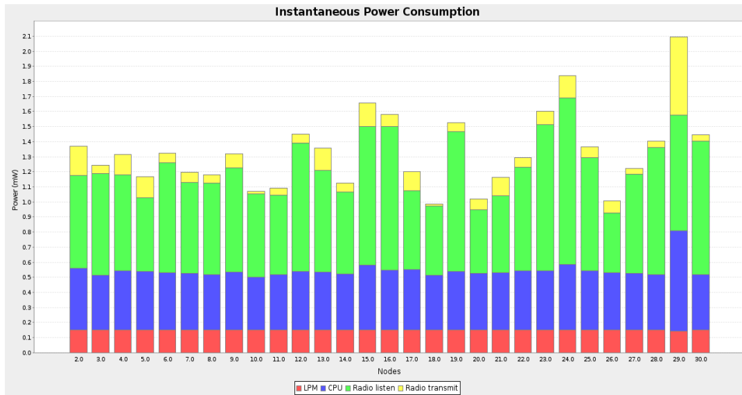
(c) – Instantaneous power consumption of 30 nodes of M_2 device
