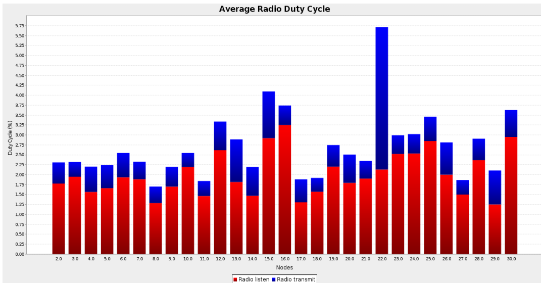
(b) – Communication power consumption of 30 nodes M_2 device
