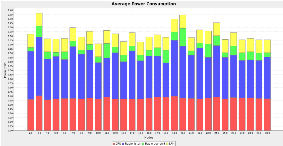
(a) – Computational power consumption of 30 nodes M_1 device
